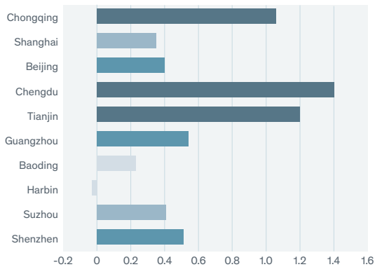
Figure 3 10 Most Populous Prefectures: Gains in Life Expectancy due to Pollution Reduction, 2013-2016
