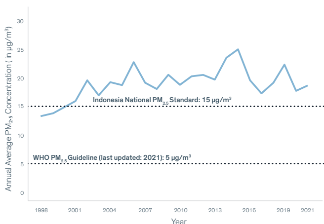
Figure 4 · Annual average PM 2.5 concentration in Indonesia, 1998-2021
